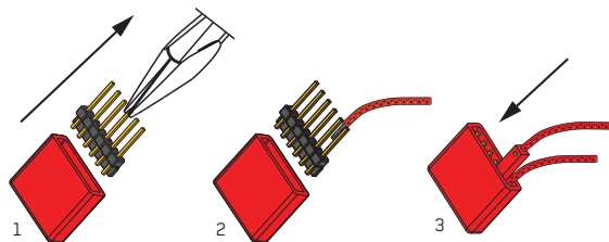
Solder the RED wire from the Battery Holder and/or pickups and re-insert the Header into the insulation cover
