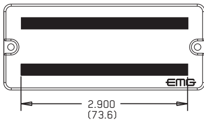
EMG-35CS/DC
