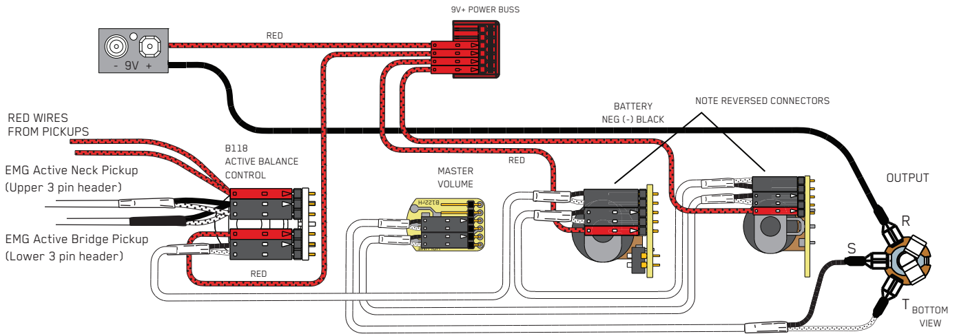
Diagram #5 ABC Balance Control Master Volume VMC Control Output Jack
