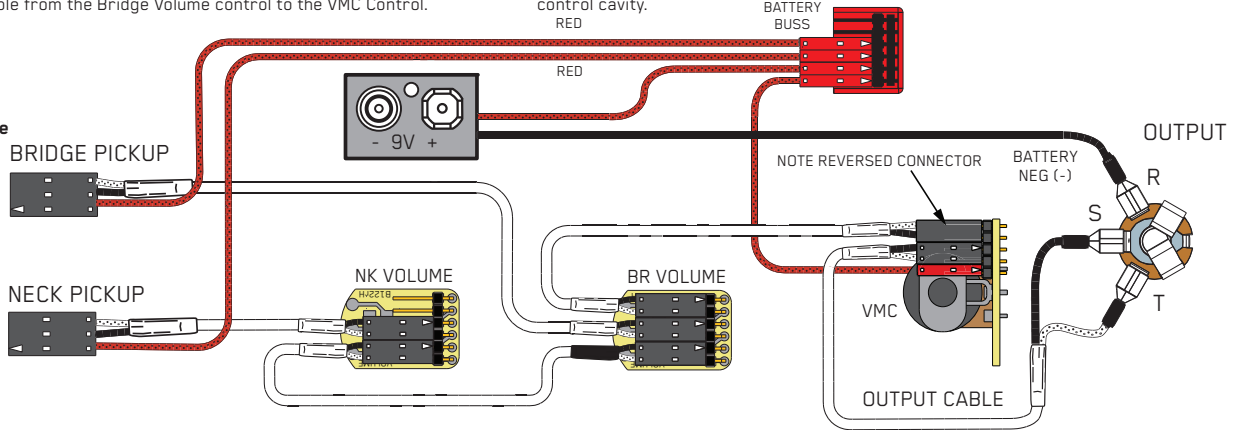
Diagram #3 Volume / Volume VMC Control
