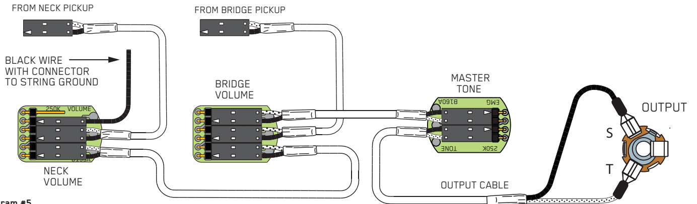
Diagram #5 2 Pickups Volume / Volume/ Tone
