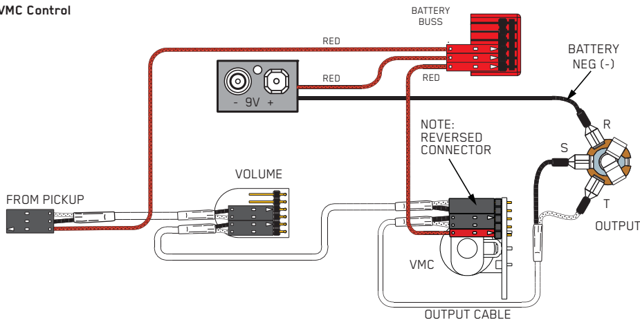
Diagram #2 Master Volume VMC Control
