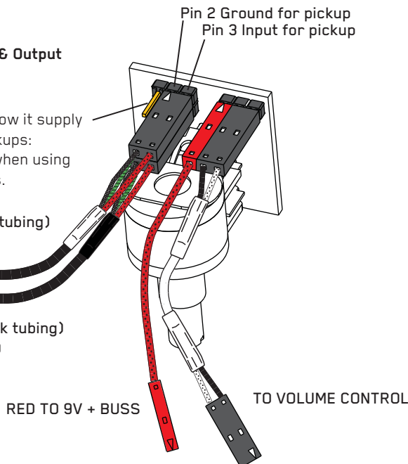
Diagram #2 EMG-HZ Pickups Soldered Inputs
